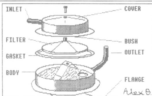
Fig. 3.1. Fuel Pump
